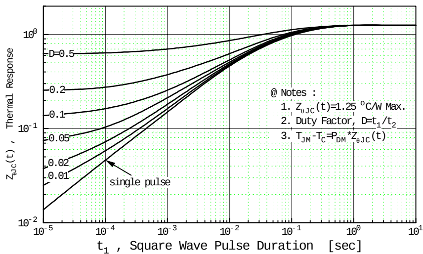
Fig. 11 Thermal Response
